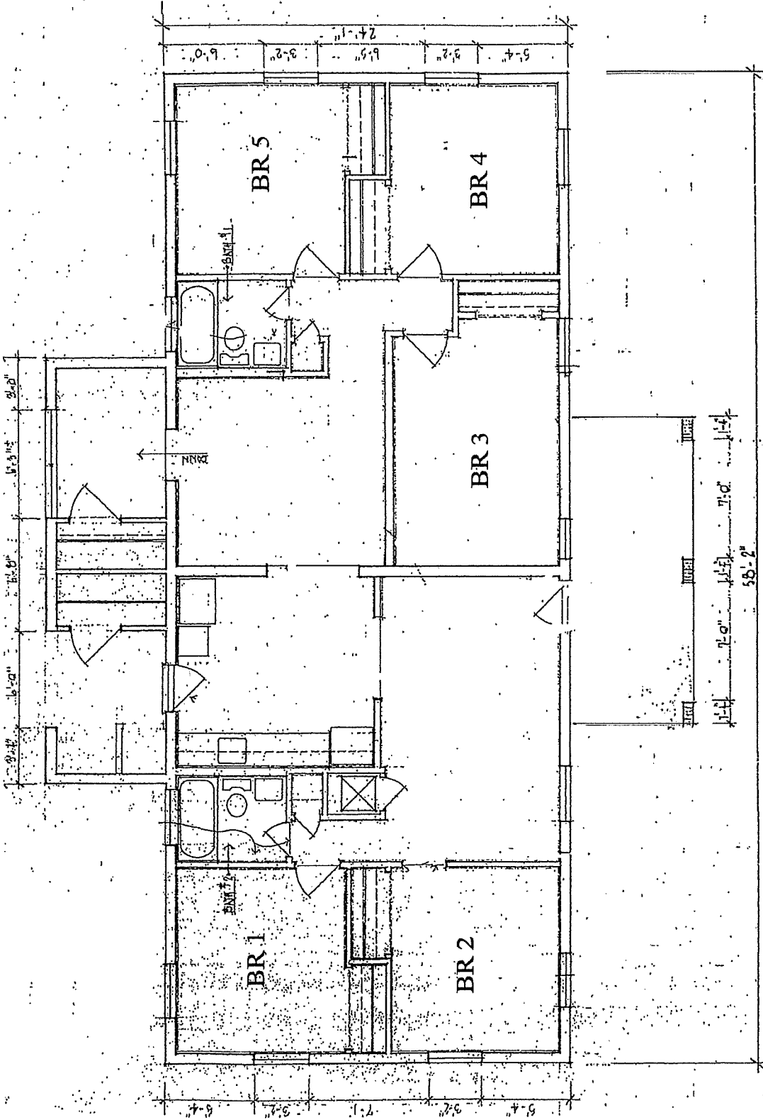
FLOOR PLAN 1119 NE 26th Terrace
